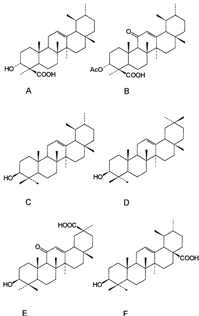
Fig. 1. Chemical structures of the pentacyclic triterpenes used in the present study A) \beta -boswellic acid; B) AKBA; C) \alpha -amyrin; D) \beta -amyrin; E) 18 \beta -glycyrrhetic acid; F) ursolic acid).
