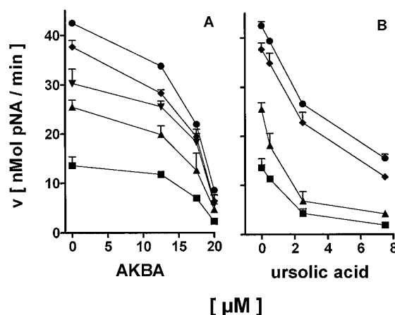
Fig. 2. Inhibition of HLE activity by AKBA (panel A) and ursolic acid (panel B). Substrate (MeO-Suc-Ala-Ala-Pro-Val-pNA) concentrations were 50 ( \blacksquare ), 100 ( \blacktriangle ), 150 ( \blacktriangledown ), 300 ( \blacklozenge ) and 500 \mu\text{M} ( \bullet ). The assays were carried out in PBS/10.25% DMSO, pH 7.2, at 25°C. The enzyme concentration was 20 nM. Data are shown as absolute values of pNA release, in nanomoles per minute, as means \pm S.D. of three experiments.
